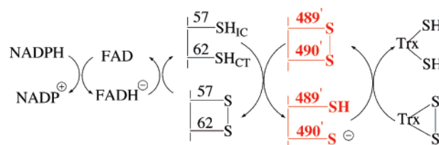
FIGURE 1: Proposed pathway for transfer of electrons to Trx by DmTR. Cys57 is the interchange residue (Cys57 IC ), and Cys62 is the charge-transfer residue (Cys62 CT ). Once Cys57 becomes reduced by the flavin cofactor, it initiates attack on the 8-membered ring formed by adjacent Cys residues on the C-terminus on the opposing subunit. The reduction of this 8-membered ring is the additional thiol–disulfide exchange step not found in GR. We refer to this step in the reaction mechanism as the ring-opening step, and it is highlighted in red in the diagram. Once this ring is reduced, the attacking nucleophile (Cys490') initiates attack on the disulfide bond of Trx. The prime designation indicates residues that are on the adjacent subunit.
