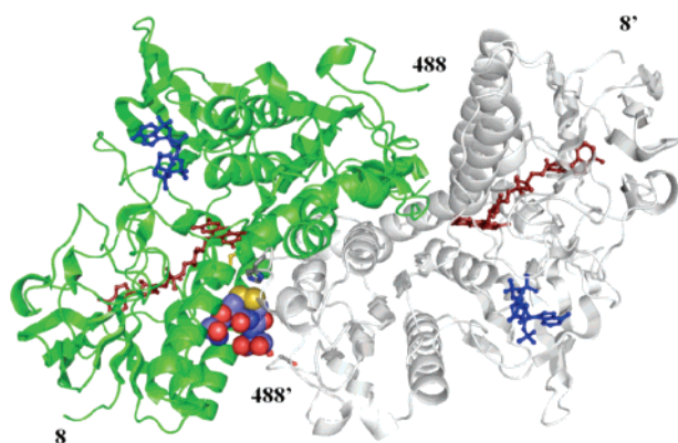
FIGURE 2: Crystallographic structure of the TR from Drosophila . The homodimeric model of DmTR with chain A is shown in green and chain B is shown in gray. The SCCS(ox) tetrapeptide in the C+ is oriented with Cys489' as the interchange residue and is shown in space-filling model format. NADP without the nicotinamide moiety is indicated in blue and FAD in dark red. The prime designation for residue numbers indicates the B chain of the TR homodimer, and the resulting images were generated in PyMOL (50).
