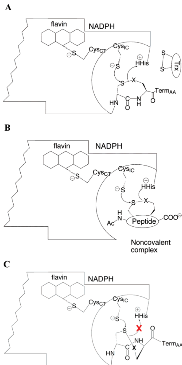
FIGURE 6: (Panel A) Diagrammatic model of one-half of the TR dimer showing the position of the C-terminal tetrapeptide as it is undergoing ring opening. Once ring opening occurs, the reduced Cys is poised to attack the disulfide bond of Trx shown to the right. If the C-terminal tetrapeptide is removed, then oxidized tetrapeptides can act as substrates for the truncated enzyme as shown in panel B and undergo a ring-opening step analogous to the step in (panel A) when the tetrapeptide is covalently attached to the enzyme. If the C-terminal peptide is in a T- conformation as shown in panel C), then proton transfer cannot take place from the catalytic His residue to the leaving-group position. Whereas in panel A, the peptide bond geometry is cis, allowing for proton transfer to the leaving group. In mammalian TRs that contain a selenium atom as the leaving group, protonation would be unnecessary. Cys IC is the interchange Cys57, and Cys CT is the charge-transfer Cys62 in DmTR, Term AA is the last amino acid of the tetrapeptide, and X is the leaving-group residue (either Cys or Sec).
