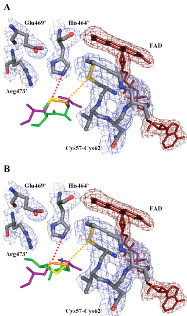
FIGURE 4: Alignment of the tetrapeptide SCCS(ox) in the structure of TR from Drosophila . The tetrapeptide structures were determined by NMR spectroscopy and placed in the tetrapeptide binding pocket of TR in accordance to the position of GSH I (the interchange position) in the GR structure (pdb 1GRA). The FAD cofactor (dark red) and the helical loop of the conserved active site sequence CVNVGC, which are components of chain A, are shown. Also shown is Arg473' from chain B as well as His464' and Glu469', which are analogous to His467' and Glu472' in GR. The oxidized C-terminal disulfide of chain B is reduced by the FAD-associated disulfide of chain A during the enzymatic cycle. The residues from TR are in gray, oxidized glutathione is in purple, the tetrapeptide is in green, and the omit electron density for the 2.4 Å structure is shown. Cys57 of DmTR is in position for interchange with GSH I and the Cys489 of the SCCS(ox) tetrapeptide, which is indicated by the orange dashed line. GSH II is in position for protonation from His464' as is Cys490' of the SCCS(ox) tetrapeptide when in the C+ conformation (Panel A) but not when in the T- conformation (Panel B) as indicated by the red dashed line. Only the cysteines for the SCCS(ox) peptide and GSSG are shown for simplicity.
