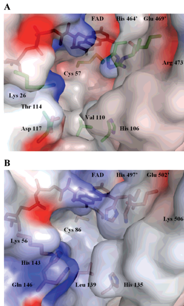
FIGURE 5: Electrostatic surface potential calculated using GRASP (52) for thioredoxin reductase showing a close-up of the tetrapeptide binding pocket, where thiol-disulfide exchange occurs between the conserved N-terminal dithiol and the C-terminal tetrapeptide of the adjacent subunit containing the 8-membered ring that must be opened during redox cycling. (Panel A) Interface for DmTR. (Panel B) Interface for mTR3 (pdb 1ZKQ).
