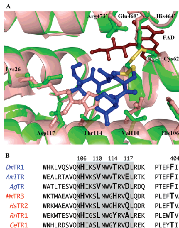
FIGURE 3: Tetrapeptide binding pocket where thiol–disulfide exchange occurs between the FAD-associated active site from chain A and the C-terminal disulfide of chain B for DmTR. Panel A is a close-up view of the SCCS(ox) tetrapeptide (blue) in the C+ conformation with Cys 489' as the interchange residue positioned in the DmTR structure (green) with an overlay of the mTR3 (pdb 1ZKQ) colored in salmon pink. Panel B is a multiple sequence alignment generated with ClustalW (51) with either the pdb ID or accession number in parentheses. Cys-containing TRs are shown in blue letters and Sec-containing TRs are shown in red letters. The sequences are TR1 from D. melanogaster (AF301144_1), TR from A. mellifera linguistica (AAP93583.1), TR from A. gambiae (CAD30858.1), TR3 from M. musculus (pdb 1ZKQ), TR2 from H. sapiens (Q9NNW7), TR1 from R. norvegicus (pdb 1H6V), and TR1 from C. elegans (AF148217_1). The alignment shows helix 3 from chain A with turns 3–6 in the shaded portion along with the loop from the dimerization domain of chain B. The numbering is in accordance with the TR from Drosophila .
